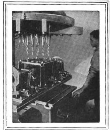
Drilling 12 stud holes at once in a worm-gear axle housing
